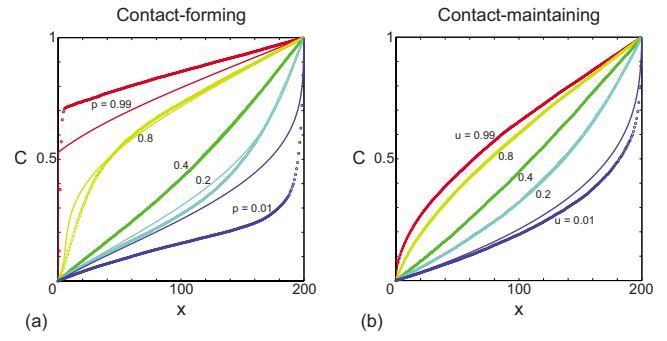
FIG. 4. (Color online) Discrete and continuum steady state results on a hexagonal tiling for (a) contact-forming interactions with s=1-p , for various values of p , and (b) contact-maintaining interactions with w=1-u for various values of u . Discrete simulations (results given by colored circle markers) are performed on a 200 \times 200 lattice with P=\Delta=\tau=1 and averages are taken over 200 Monte Carlo realizations. All simulations are performed over many time steps until the change in occupancy of all columns across the lattice is less than 0.007. The implicit solution given by Eq. (17) is shown in colored solid lines. In (a) for p=0.99 , D(C)<0 for some values of C and the solution of the continuum model has a shock at x=0 . All other plots have positive D(C) and their solutions are smooth.
