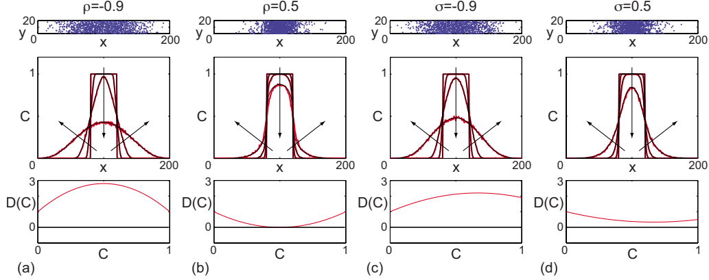
FIG. 7. (Color online) Transient results for a hexagonal tiling with biased interactions, (a) contact-forming only \rho=-0.9 , (b) contact-forming only \rho=0.5 , (c) contact-breaking only \sigma=-0.9 , and (d) contact-breaking only \sigma=0.5 . Results in the top row show the distribution of agents in a single realization after 1000 time steps. The middle row compares the solution of the continuum model (black) and the averaged column density data (red) at t=0, 10, 100, 1000 ; arrows indicate the direction of increasing time. The bottom row shows the functional dependence of D(C) on C (red) with D(C)=0 given by the horizontal line (black). All discrete data use P=\Delta=\tau=1 and averages are taken over 200 Monte Carlo realizations. Numerical solutions of the continuum models use \delta x=0.5 and \delta t=0.1 .
