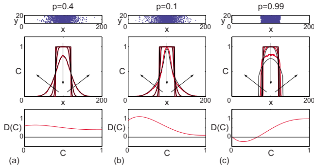
FIG. 2. (Color online) Transient results for contact-forming interactions on a hexagonal tiling ( k=3 , \beta=7 ) for various interaction strengths with s=1-p for (a) p=0.4 (mildly repelling), (b) p=0.1 (strongly repelling), and (c) p=0.99 (very strongly attracting). Results in the top row show the distribution of agents in a single realization after 1000 time steps. The middle row compares the solution of the continuum model (black) and the averaged column density data (red) at t=0, 10, 100, 1000 ; arrows indicate the direction of increasing time. The bottom row shows the functional dependence of D(C) on C (red) with D(C)=0 given by the horizontal line (black). All discrete data use P=\Delta=\tau=1 and averages are taken over 200 Monte Carlo realizations. Numerical solutions of the continuum models use \delta x=0.5 and \delta t=0.1 . In (c), D(C)<0 for some values of C and the solutions of the continuum model have a discontinuity.
