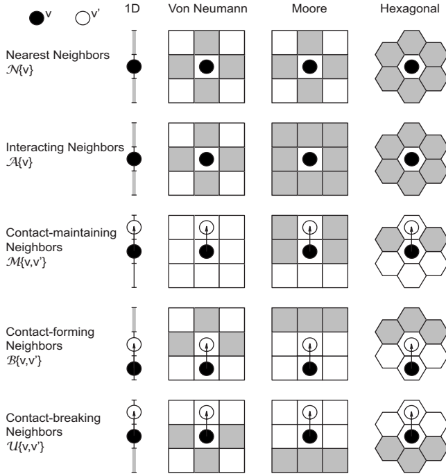
FIG. 1. Neighborhood sets for a one-dimensional and various two-dimensional lattices. Black markers depict the reference site v , white markers depict the target site v' \in \mathcal{N}\{v\} . The defined neighborhood set in each row is shaded gray. Note that in one-dimension and for the von Neumann neighborhood, \mathcal{M}\{v, v'\} = \emptyset .
