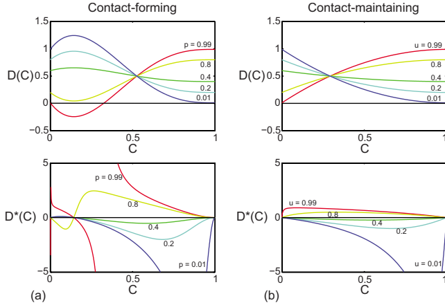
FIG. 5. (Color online) Nonlinear diffusion D(C) and dimensionless measure D^*(C) on hexagonal tiling for (a) contact-forming interactions with s=1-p for various values of p , and (b) contact-maintaining interactions with w=1-u for various values of u .
