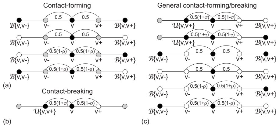
FIG. 6. Probability bias on a one-dimensional lattice. Black markers represent occupied sites, white represent unoccupied, and gray represent sites that are independent of the bias interaction rules. The factor P/L has not been shown here. (a) The contact-forming interaction probabilities, (b) the contact-breaking interaction probabilities, and (c) the general contact-forming and contact-breaking interaction probabilities. Here, -1 \leq \rho, \sigma, \gamma \leq 1 .
