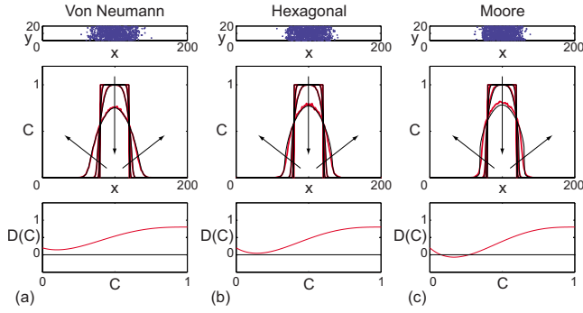
FIG. 3. (Color online) Transient results for contact-forming interactions for various cases with s=1-p and p=0.8 for (a) square lattice with von Neumann interacting neighborhood ( k=3 , \beta=5 ), (b) hexagonal tiling ( k=3 , \beta=7 ), and (c) square lattice with Moore interacting neighborhood ( k=3 , \beta=9 ). Results in the top row show the distribution of agents in a single realization after 1000 time steps. The middle row compares the solution of the continuum model (black) and the averaged column density data (red) at t=0, 10, 100, 1000 ; arrows indicate the direction of increasing time. The bottom row shows the functional dependence of D(C) on C (red) with D(C)=0 given by the horizontal line (black). All discrete data use P=\Delta=\tau=1 and averages are taken over 200 Monte Carlo realizations. Numerical solutions of the continuum models use \delta x=0.5 and \delta t=0.1 . In (c), D(C)<0 for some values of C and the solutions of the continuum model have a discontinuity.
